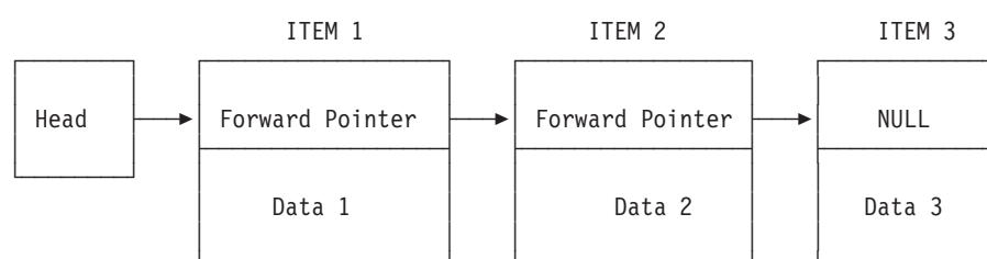
Figure 17. Example of one-directional chain
